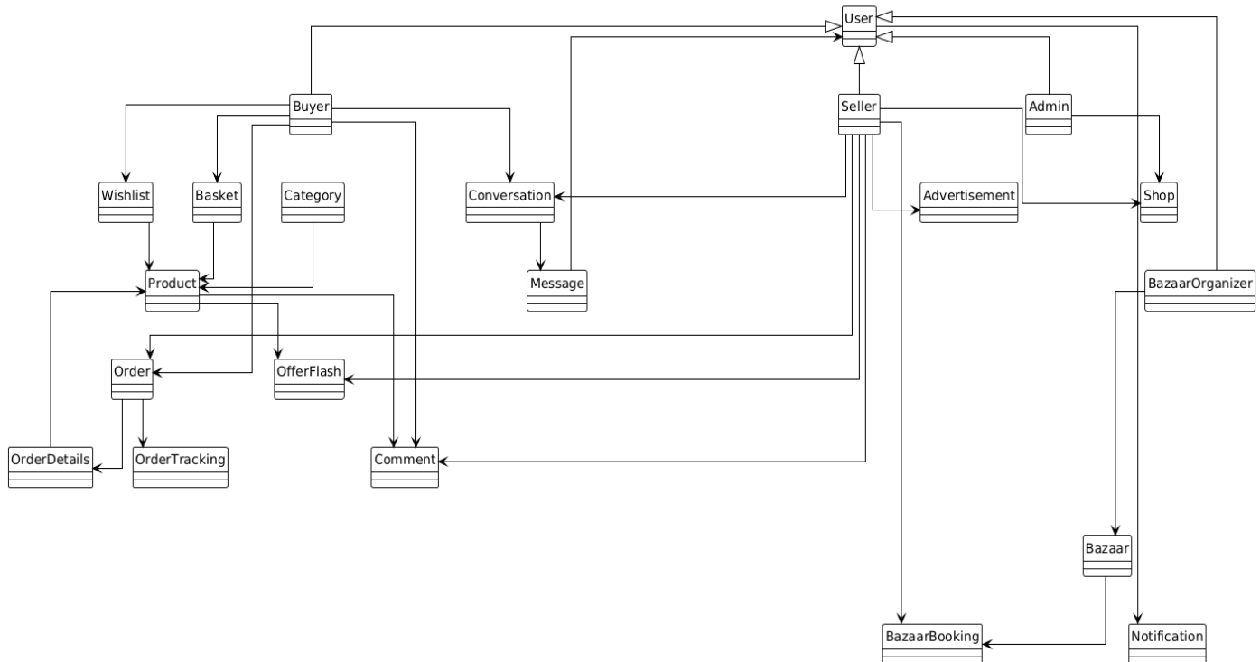
Figure 76 High level class diagram
