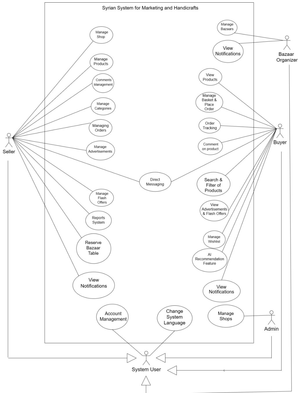
Figure 3: High level-use case diagram
