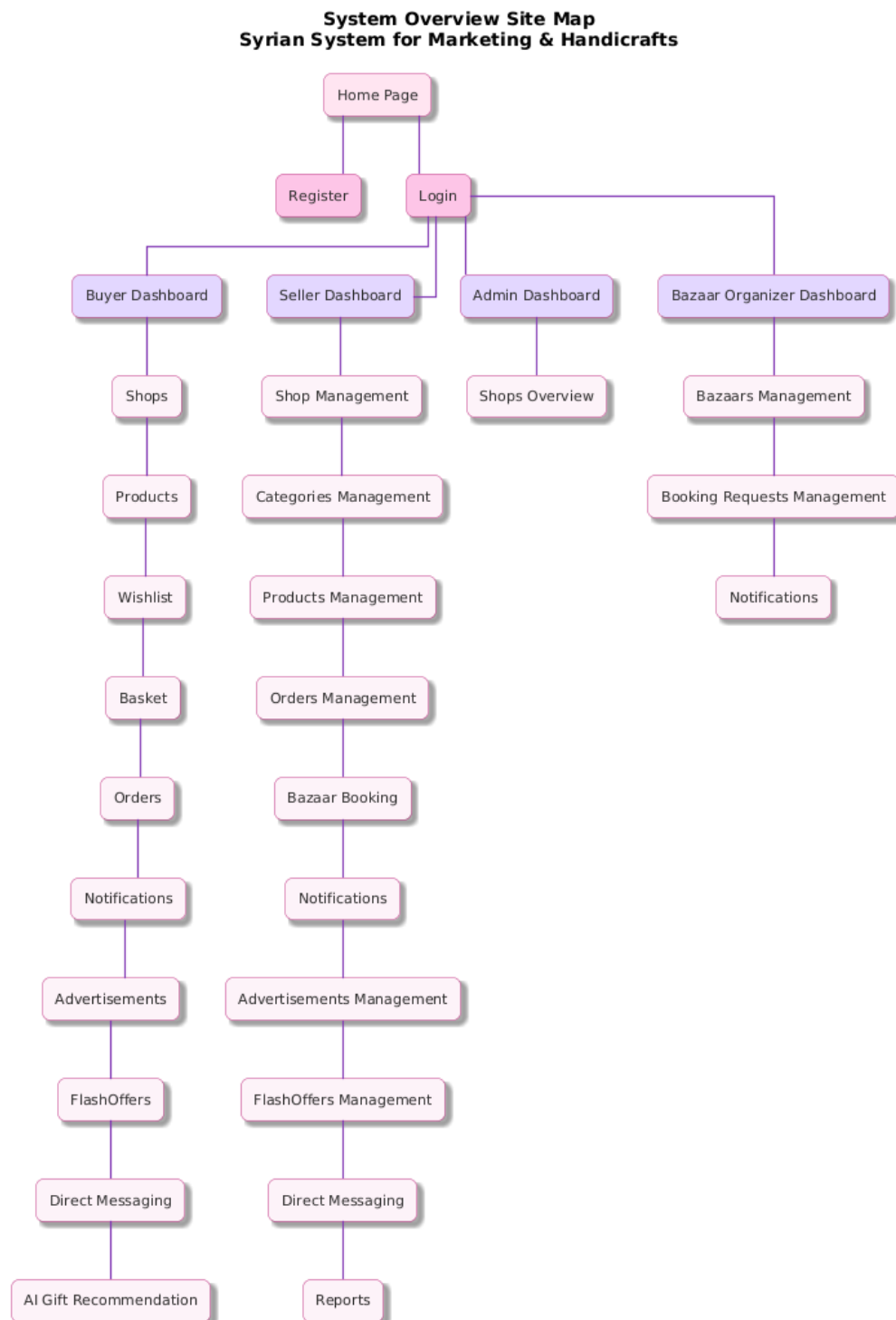
Figure 92 System Overview Site Map
