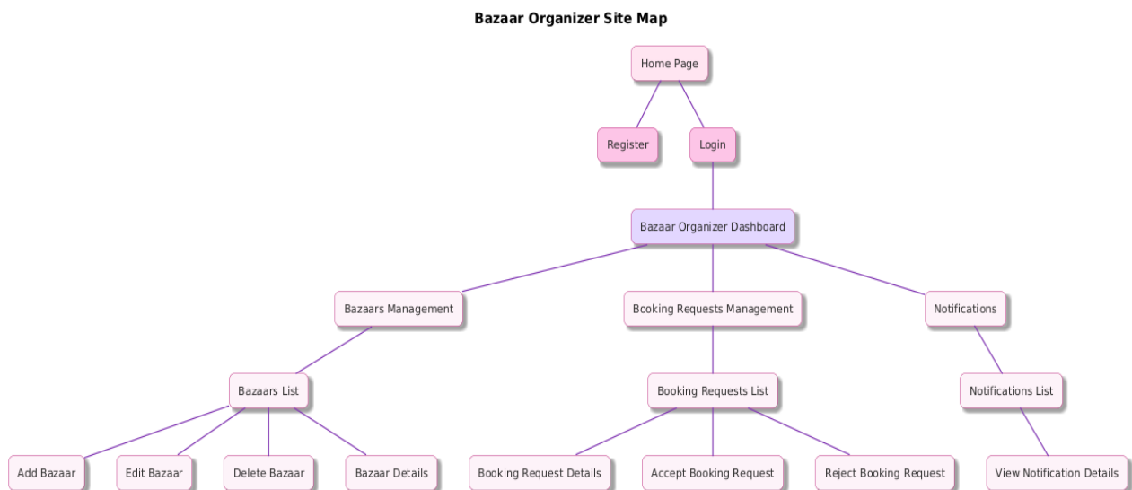
Figure 96 Bazar Organizer Site Map
